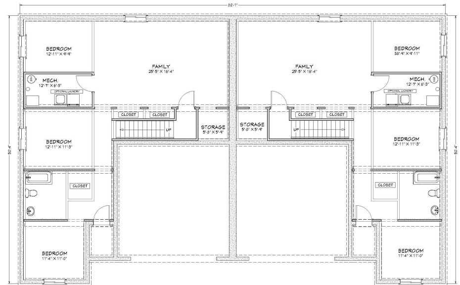
Proposed Finished Basement
