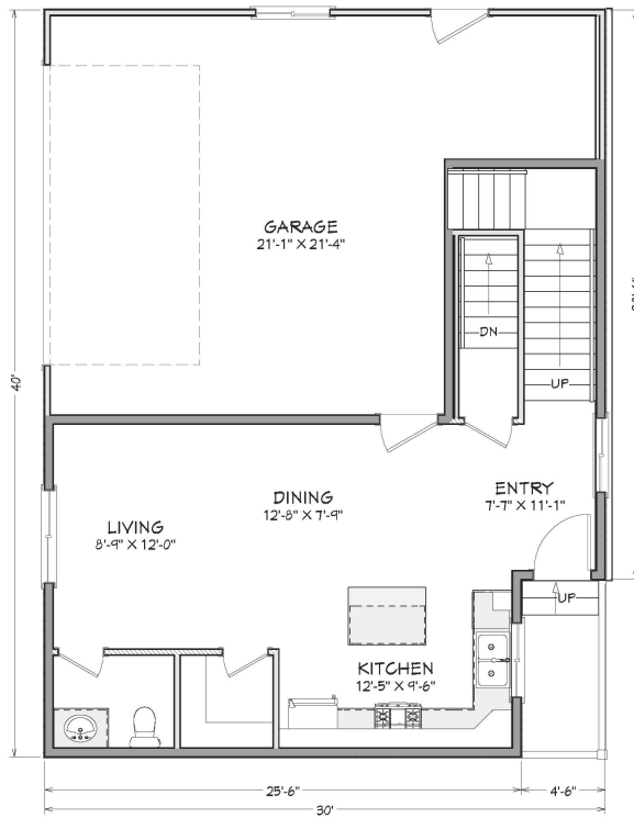
Main Floor
