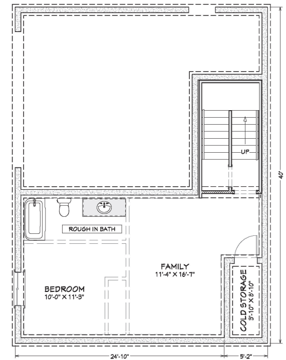
Proposed Basement
