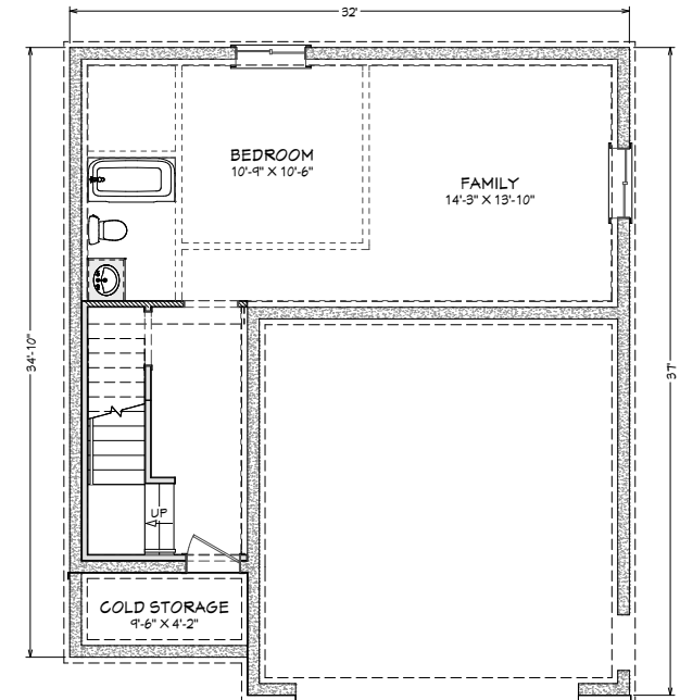
Proposed Basement
