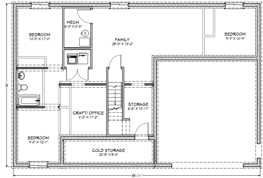
Second Floor
